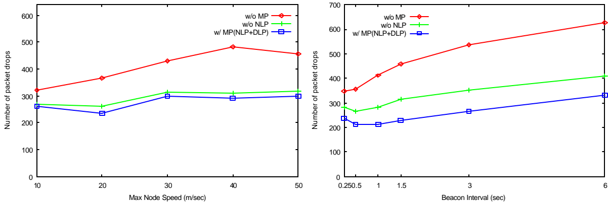
(a) Drop by ARP under RWP mobility
