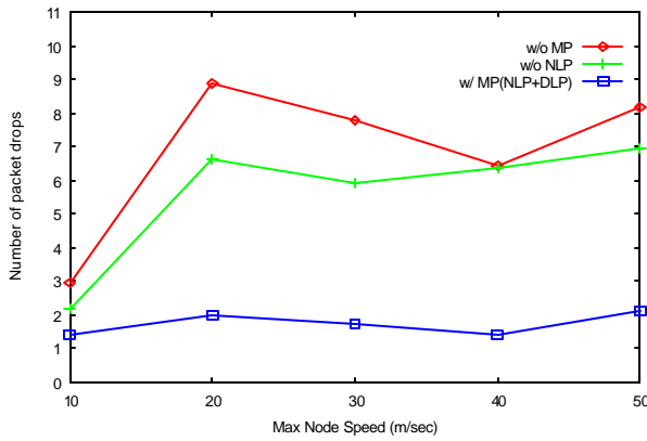
(a) Drop by TTL under RPGM mobility
