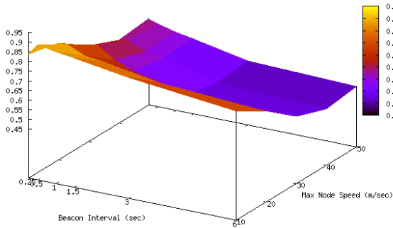
(a) SDR without MP (RPGM model)
