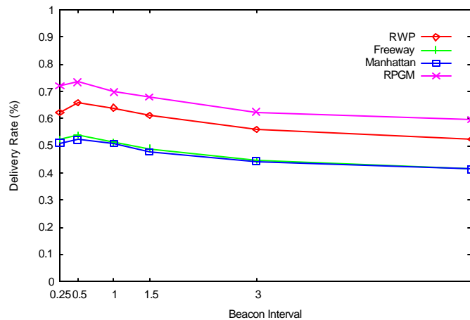
Figure 5. SDR varying beacon interval
