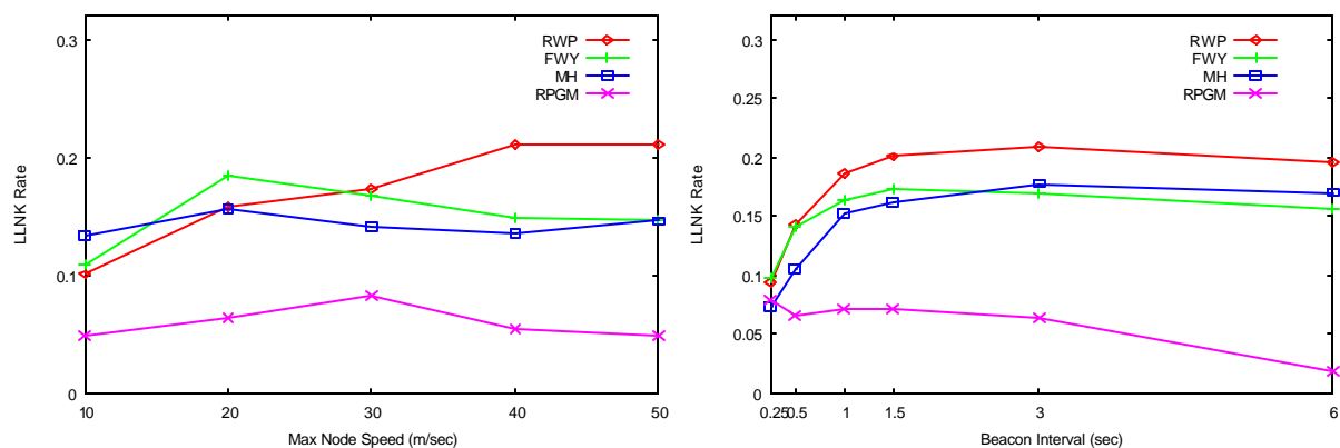
Figure 9. Percentages drop in LLNK with NLP scheme. The higher value in each graph indicates the more savings from LLNK with NLP scheme.
