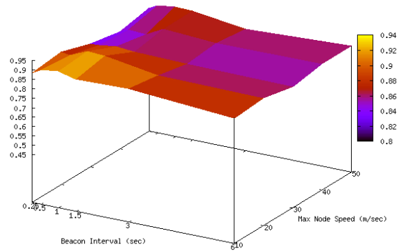
(b) SDR with MP (RPGM model)
