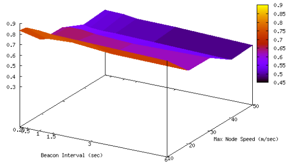
(b) SDR with MP (FWY model)
