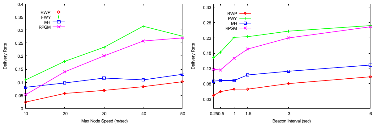
Figure 12. The improvement in SDR with MP (NLP plus DLP) scheme.
