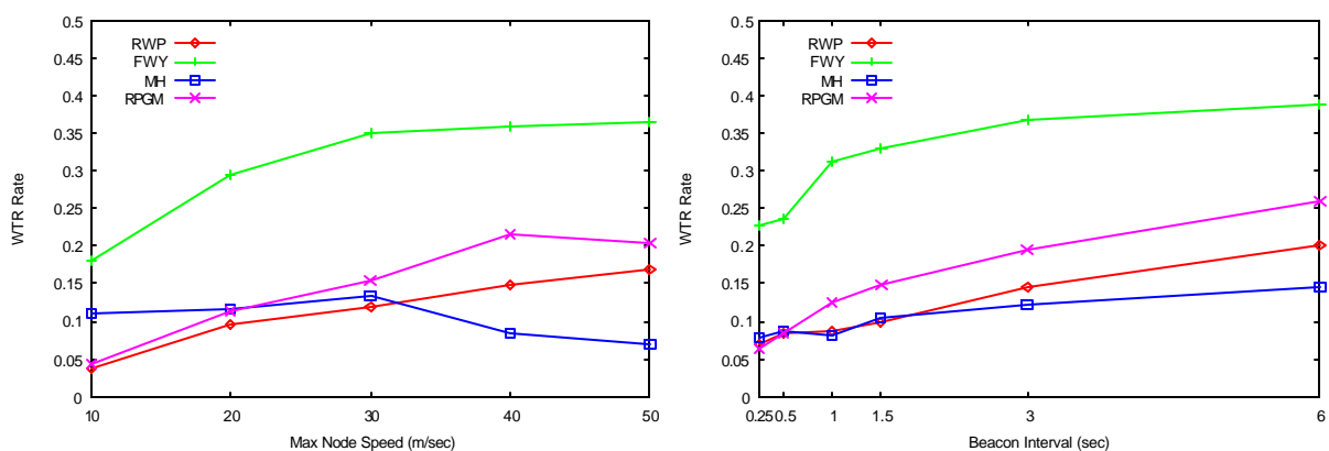
Figure 10. The reduction in WTR with DLP scheme. The value in each graph indicates additional savings in WTR with DLP scheme in addition to NLP scheme.
