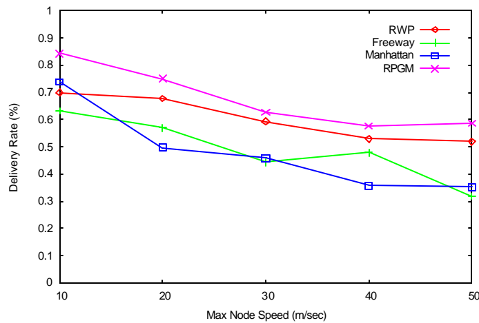
Figure 3. SDR varying maximum node speed
