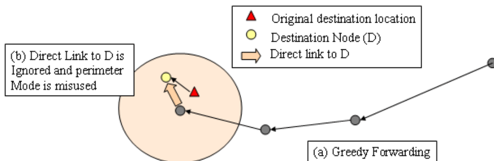
Figure 8. An example case of LOOP problem
