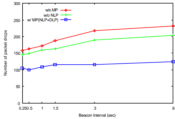
(b) Drop by NRTR under Manhattan mobility
