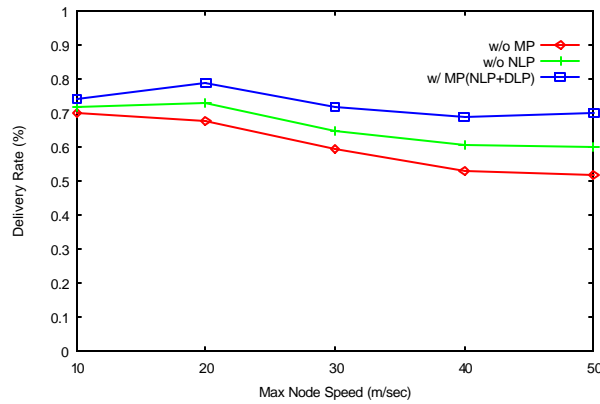
(a) SDR under RWP
