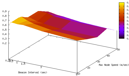
(a) SDR without MP (MH model)
