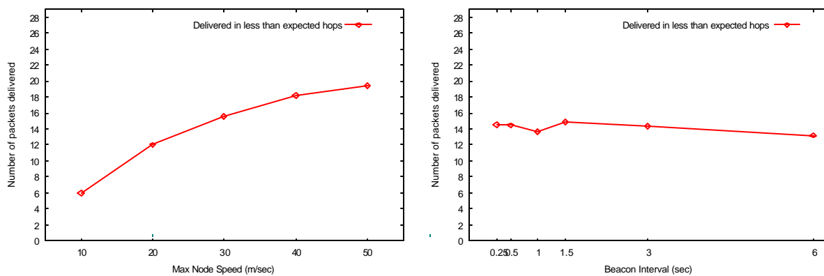
Figure 4. Number of packets delivered in less than expected hops
