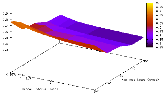
(a) SDR without MP (FWY model)
