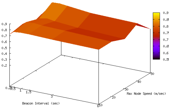
(b) SDR with MP (MH model)
