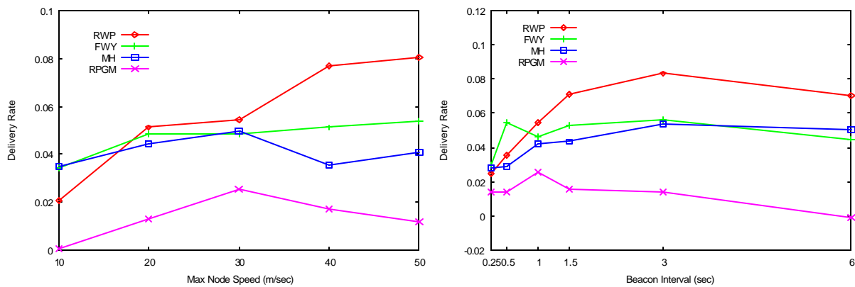
Figure 11. The improvement in SDR with NLP scheme.
