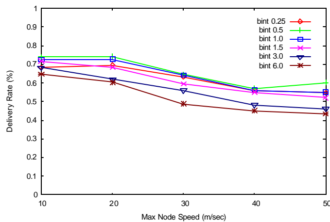
Figure 6. Effect of node mobility, beacon interval (RWP mobility)
