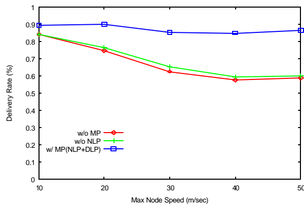
(c) SDR under MH
