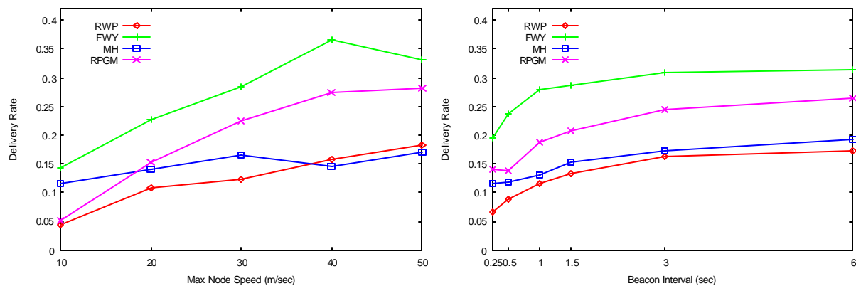
Figure 14. The improvement gained in SDR with mobility prediction scheme. The value in each graph indicates the SDR improvement from the original geographical routing scheme without mobility prediction.
